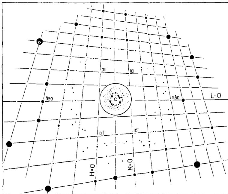
Fig. 1.—Gnomonic projection of Laue photograph made with incident beam inclined about 3^\circ from normal to (110); distance from crystal to plate, 5 cm. The scale is obtainable from the fact that the circle around the diagrammatic Laue photograph has a diameter of 10 cm.
